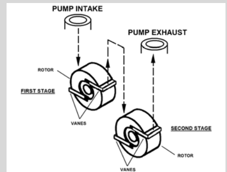
First stage exhausts into the intake of the second stage similar to two single stage pumps connected together.
